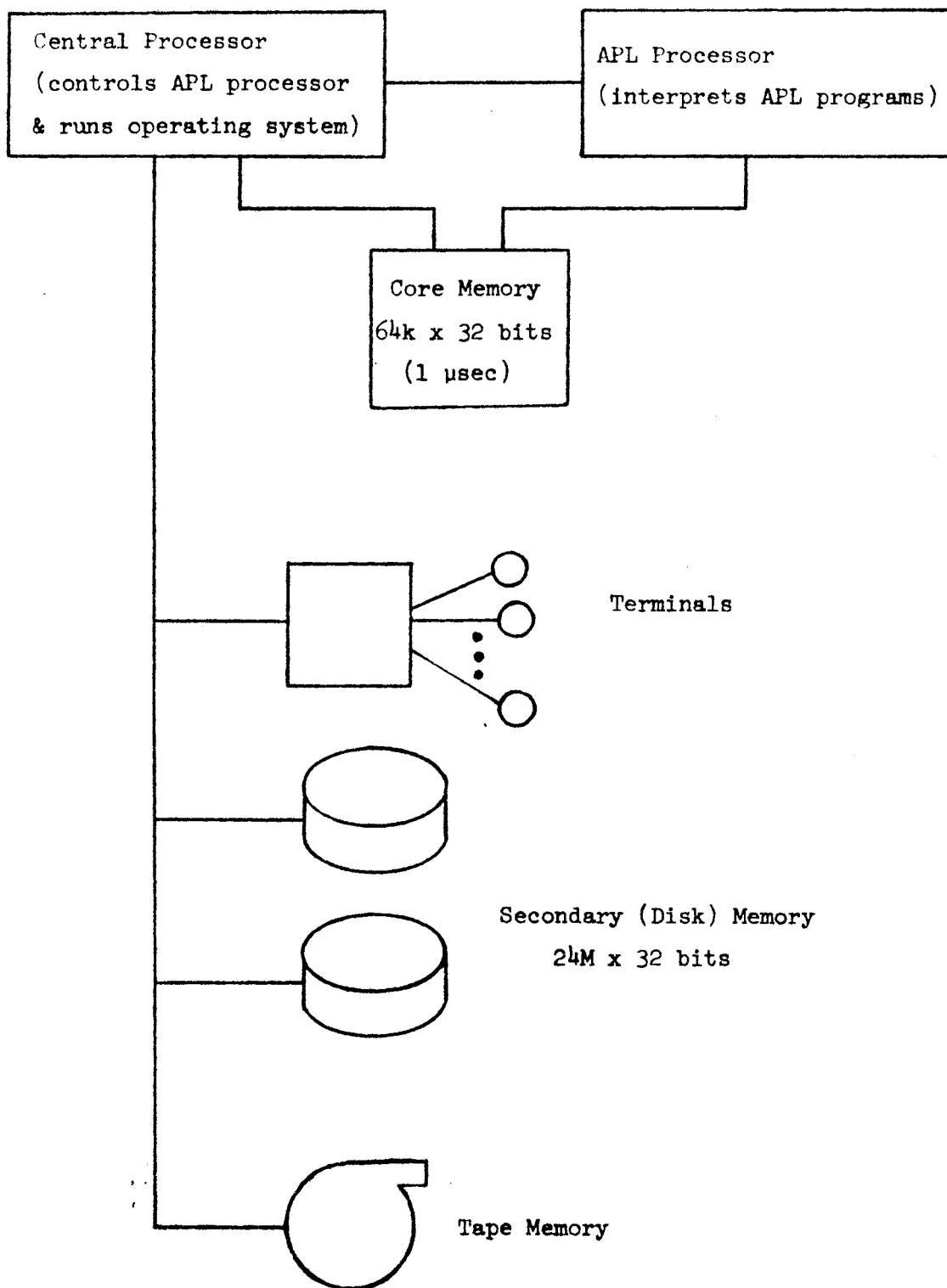
Figure 1. CRMS Computer System Configuration
